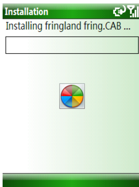
Figure 4 - Installation
